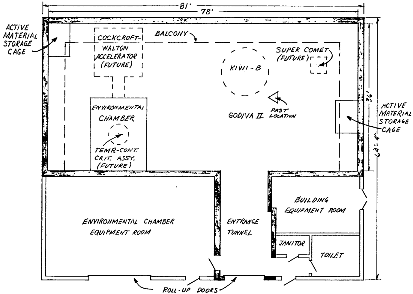
Figure 12. Kiva 3 floor plan
