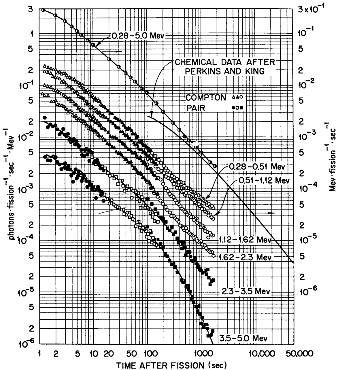
Figure 15. Time distribution of delayed gamma energy from fission fragments (from reference 14)
