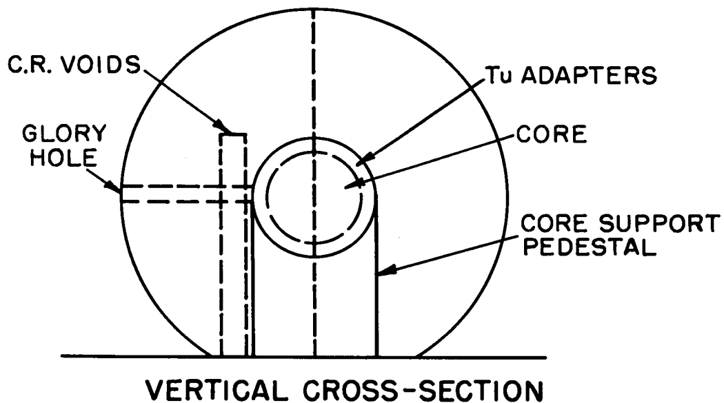
Figure A-1. Flat top schematic
