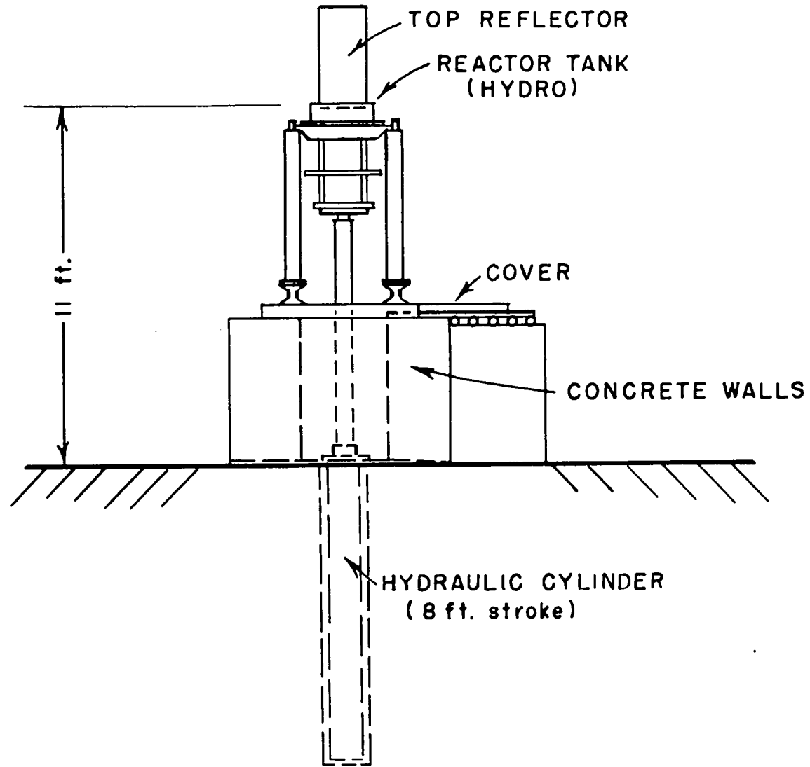
Figure 11. Hydro in outdoor facility
