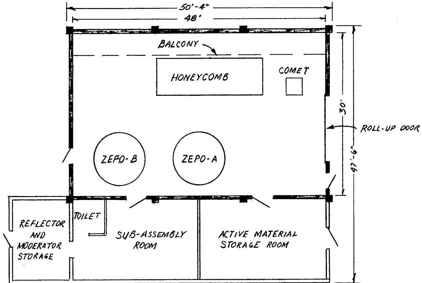
Figure 4. Kiva 1 floor plan
