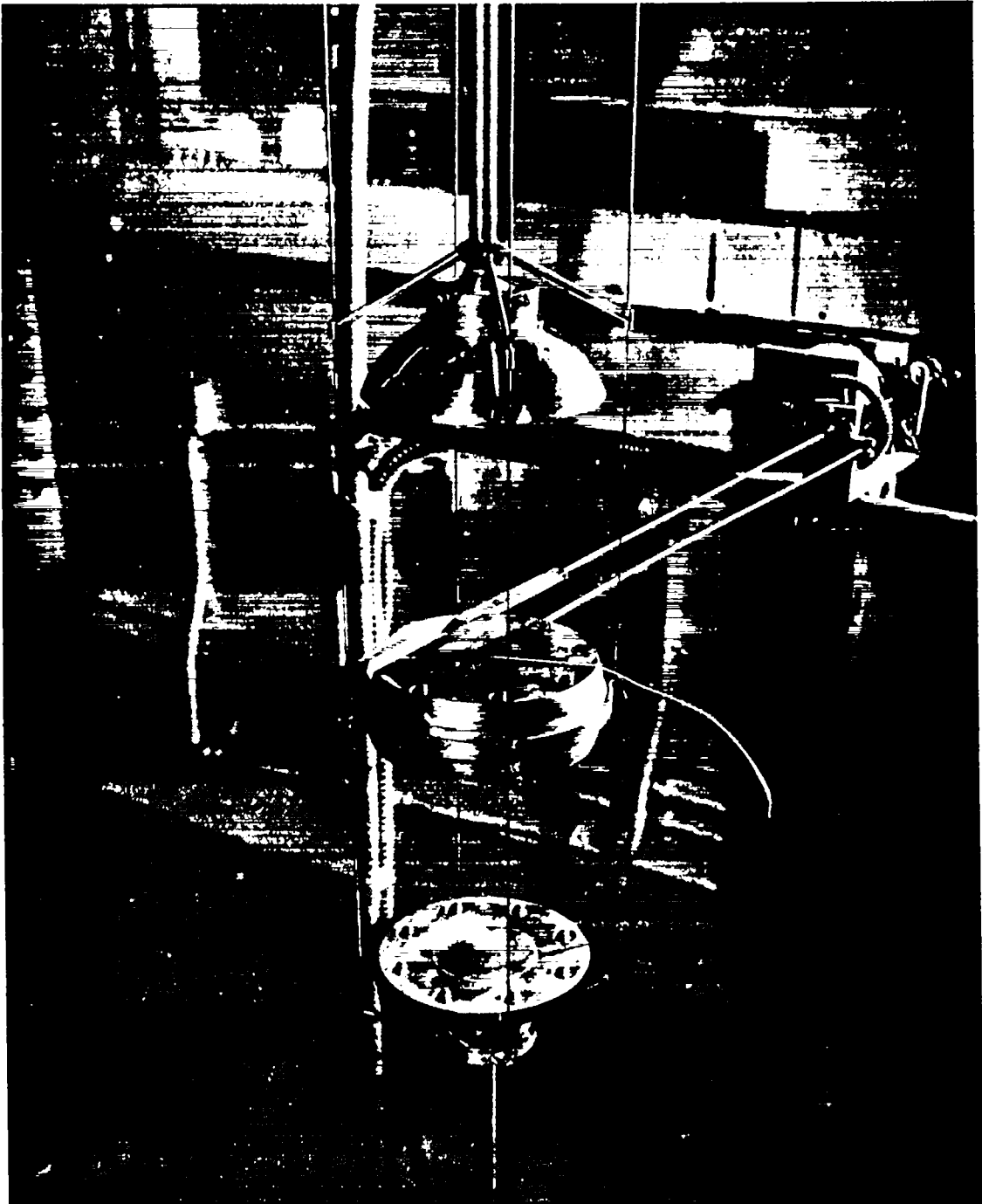
Figure 8. Jezebel in Kiva 2
