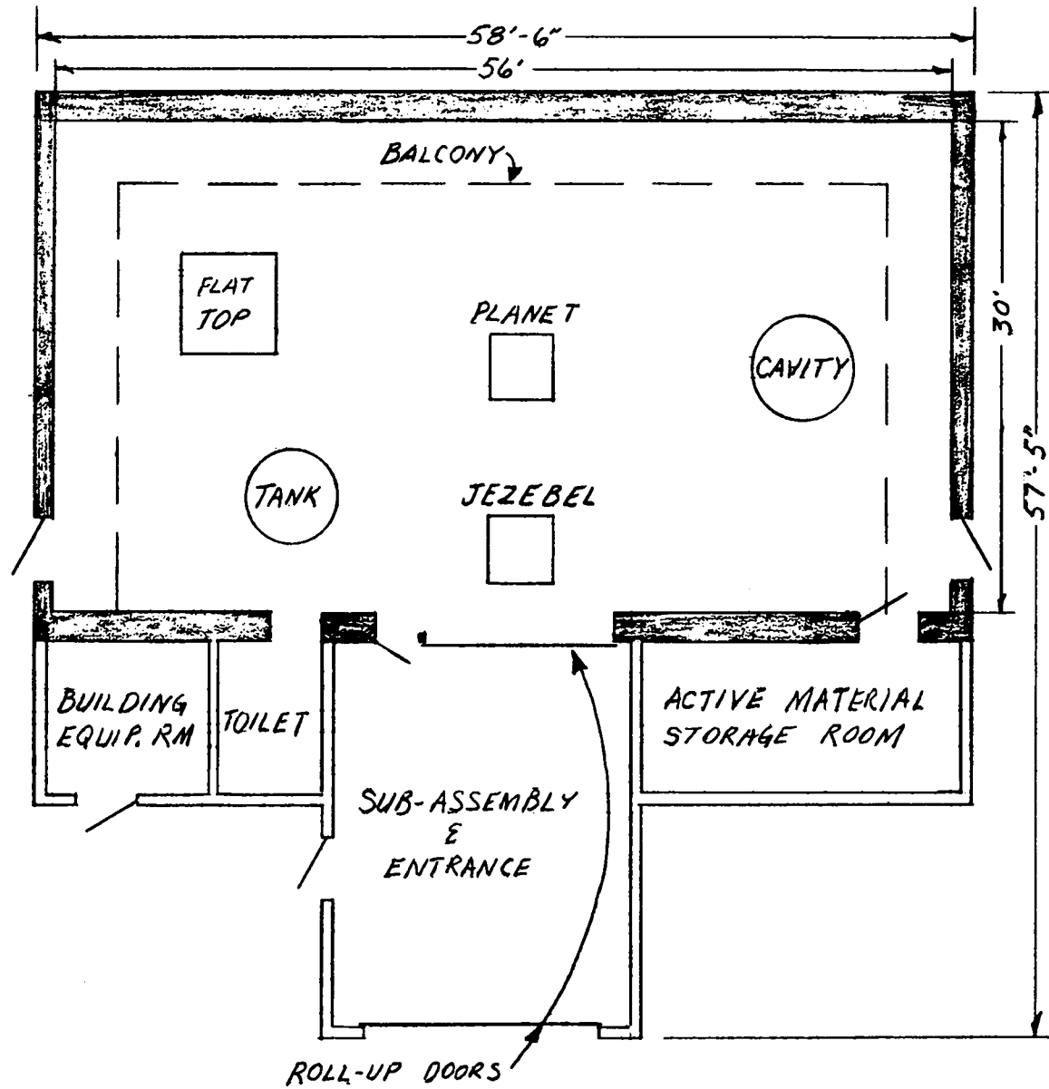
Figure 7. Kiva 2 floor plan
