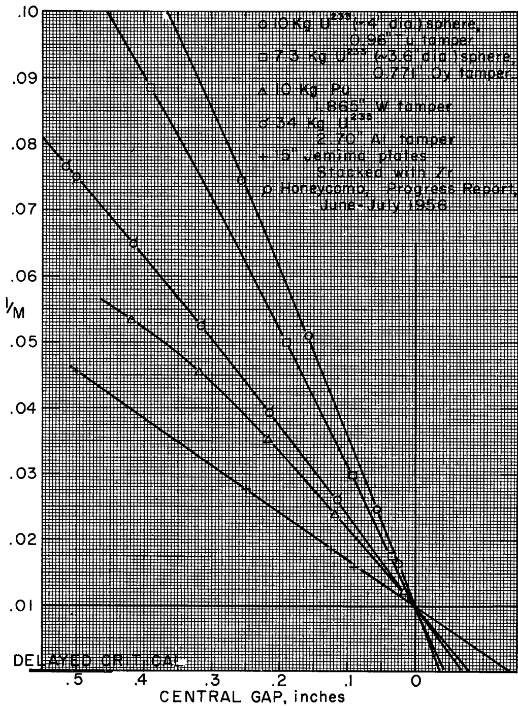
Figure 14. Dependence of reciprocal multiplication upon width of central gap in various assemblies.
