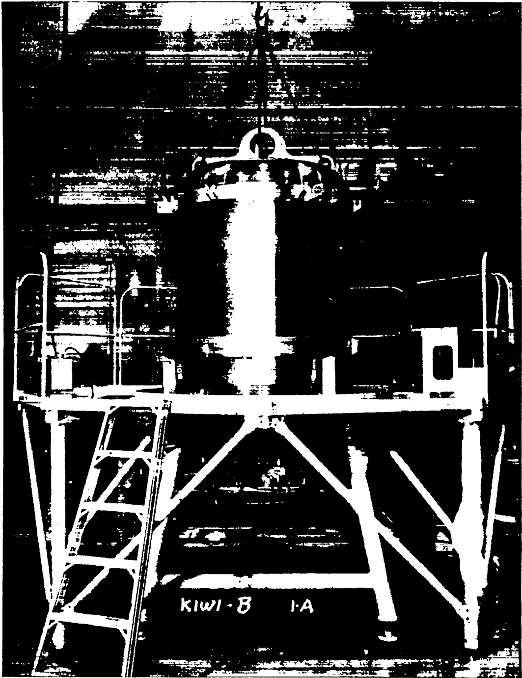
Figure 13. Kiwi-B reactor in Kiva 3
